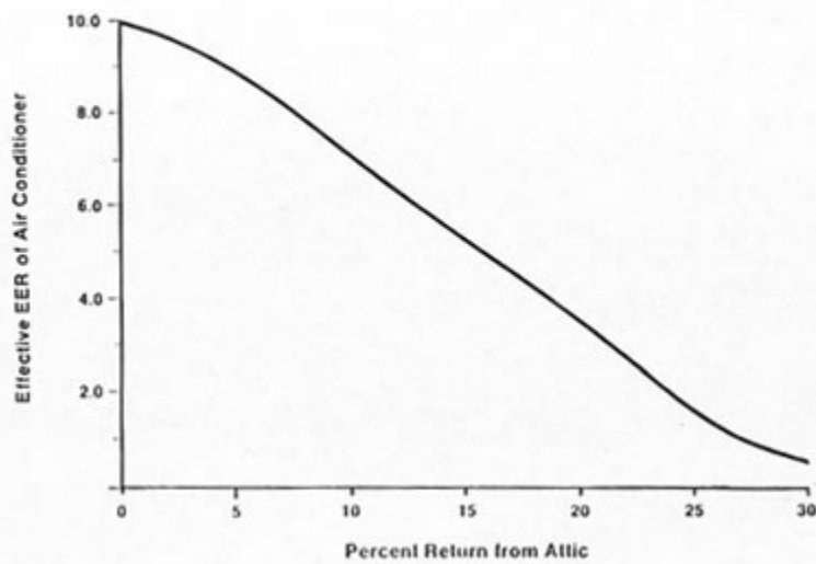
Figure 12. Degradation in air conditioner efficiency (Energy Efficiency Ratio) when various sized return leaks draw hot air from the attic, assuming the room is 78°F and attic air is 120°F.
