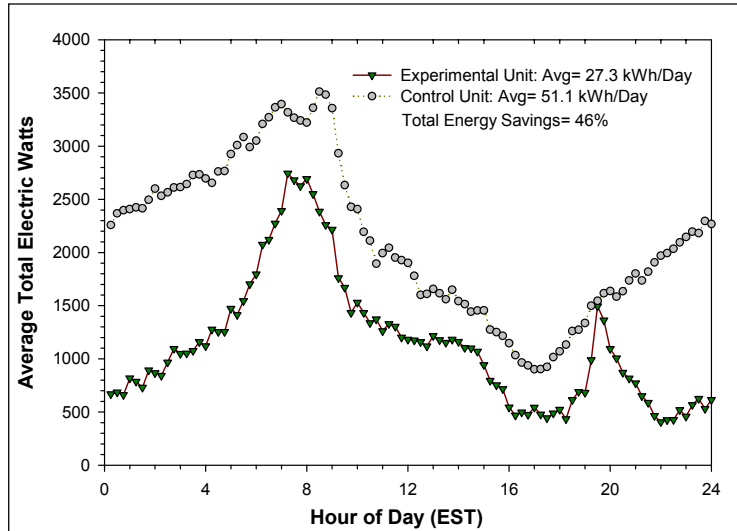
Figure 5. Electric Demand Profile November 1, 2003 – May 12, 2004, Chapel Hill, NC
