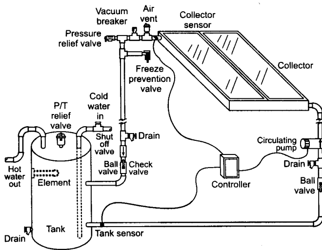
Figure 1. A solar water heating system
