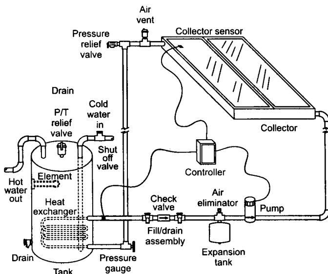
Figure 3. Indirect pumped system using antifreeze solution
