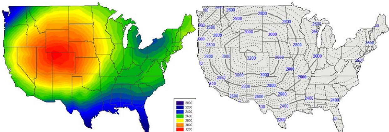
Figure 7. Annual absolute energy savings in kWh for E64FPCL
