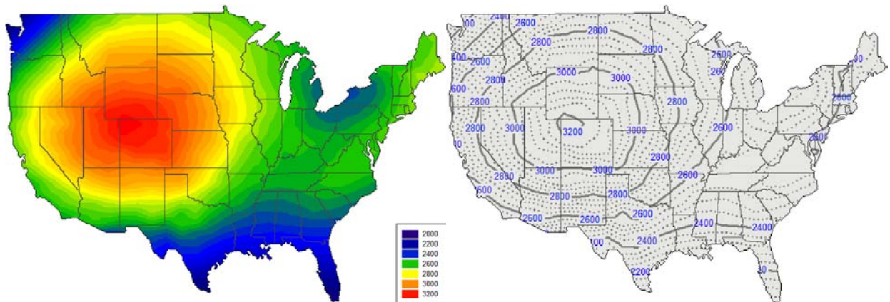
Figure A6. Annual absolute energy savings in kWh for E64FPCL
