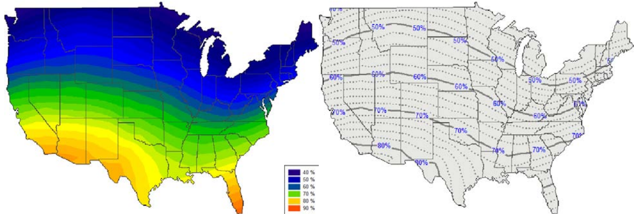
Figure E.1: Annual fractional energy savings (%) for a standard 40 gallons electric water heater combined with a 40ft 2 flat plate closed loop solar water heater
